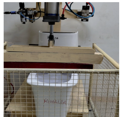
Load Bearing Test
