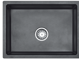
QI-004 • Single Bowl Sink Overall Size : 610x457x203mm (24"x18"x8") Bowl Size : 557x405mm Available Colors : Metallic / Advance
