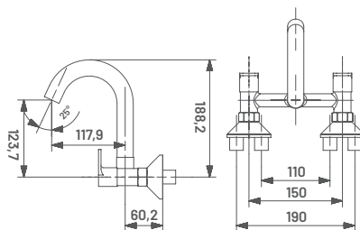
HE231 M.R.P. ₹ : 5125/- Sink Mixer (Wall Mounted) with Dual Flow Spout
