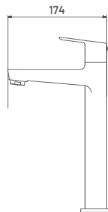
TY24 M.R.P. ₹ : 4295/- Single Lever Medium Pillar Cock with Long Nose (Lifting Type Cold Water Cartridge)
